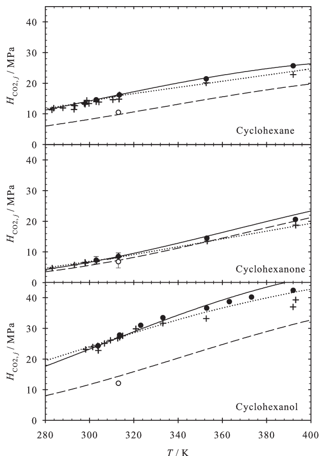
Figure 5. From top to bottom: Henry's law constant of carbon dioxide in cyclohexane, in cyclohexanone, and in cyclohexanol: + experimental data 5,7,45,46,63–67 ; ○ present simulation data with \xi = 1 ; ● simulation data with \xi = 0.95 , 0.985, and 0.918 6,7 ; - - - COSMO-SAC; — COSMO-SAC with I_{ij} = -0.0523 , -0.0082 , and -0.0418 ; ... PR EOS with k_{ij} = 0.217 , 0.049, and 0.225.
