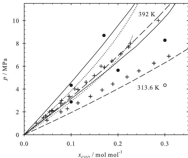
Figure 8. Isothermal vapor-liquid phase diagram (saturated liquid line only) of carbon dioxide + cyclohexanol at 313.6 and 392 K: + experimental data 5,62 ; o present simulation data with \xi = 1 ; • simulation data with \xi = 0.918 6 ; - - COSMO-SAC; — COSMO-SAC with l_{ij} = -0.0418 ; ... PR EOS with k_{ij} = 0.225 .
