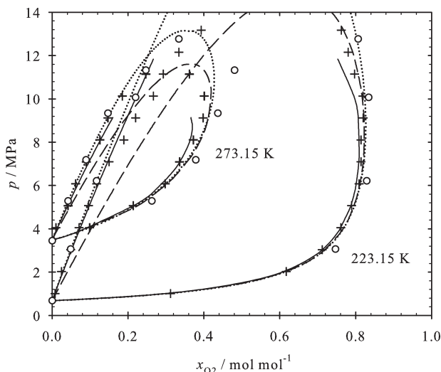
Figure 3. Isothermal vapor-liquid phase diagram of oxygen + carbon dioxide at 223.15 and 273.15 K: + experimental data 44 ; o present simulation data with \xi = 1 ; - - COSMO-SAC; — COSMO-SAC with l_{ij} = -0.0526 ; ... PR EOS with k_{ij} = 0.132 .
