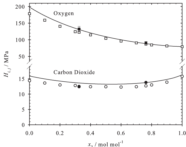
Figure 16. Henry's law constant of either ■ oxygen (1) or ● carbon dioxide (2) in the ternary mixture of cyclohexane (3) + cyclohexanone (4) + cyclohexanol (5) at 313.6 K. The gas free composition of the solvent is varied so that x'_4 = x'_5 , where x'_4 = x'_5 = 1 - x'_3 : (full symbols) present experimental data; (open symbols) present simulation data; — COSMO-SAC.
