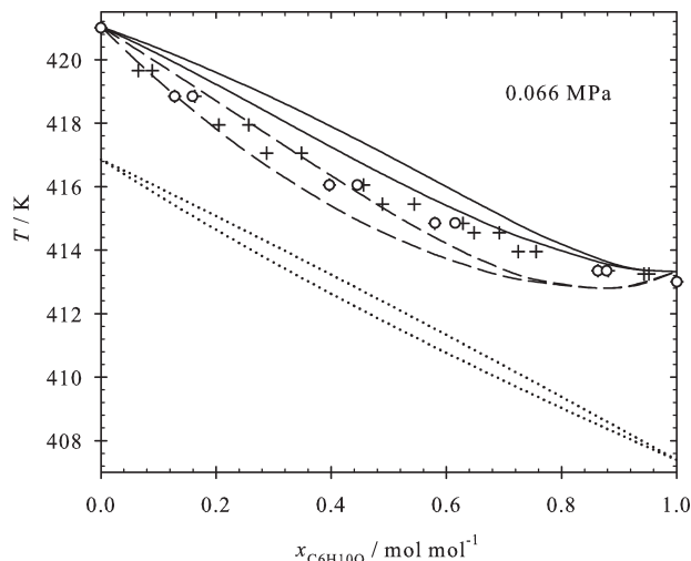
Figure 12. Isobaric vapor-liquid phase diagram of cyclohexanone + cyclohexanol at 0.066 MPa: + experimental data 71 ; ○ present simulation data with \xi = 1 ; - - - COSMO-SAC; — COSMO-SAC with I_{ij} = -0.0027 ; ... PR EOS with k_{ij} = 0 .
