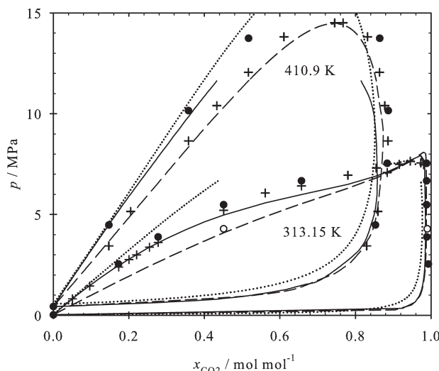
Figure 6. Isothermal vapor-liquid phase diagram of carbon dioxide + cyclohexane at 313.15 and 410.9 K: + experimental data 5,8,68 ; ○ present simulation data with \xi = 1 ; ● simulation data with \xi = 0.95 ; - - COSMO-SAC; — COSMO-SAC with I_{ij} = -0.0523 ; ... PR EOS with k_{ij} = 0.217 .
