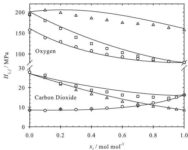
Figure 13. Henry's law constant from present simulations of oxygen (top) and of carbon dioxide (bottom) at 313.6 K in binary liquid mixtures of: ○ cyclohexane + cyclohexanone plotted over the cyclohexane mole fraction; □ cyclohexane + cyclohexanol plotted over the cyclohexane mole fraction; Δ cyclohexanone + cyclohexanol plotted over the cyclohexanone mole fraction; + experimental data 5 ; — COSMO-SAC.
