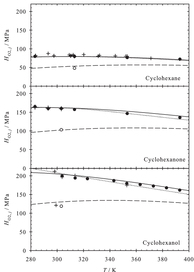
Figure 4. From top to bottom: Henry's law constant of oxygen in cyclohexane, in cyclohexanone, and in cyclohexanol: + experimental data 5,7,45,46,59–61 ; o present simulation data with \xi = 1 ; • present simulation data with \xi = 0.91, 0.93 , and 0.90 ; - - COSMO-SAC; — COSMO-SAC with l_{ij} = -0.0547, -0.0342 , and -0.0266 ; ... PR EOS with k_{ij} = 0.22, 0.255 , and 0.345 .
