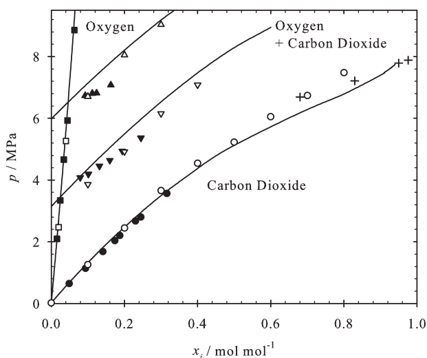
Figure 15. Solubility pressure of oxygen (1) and of carbon dioxide (2) in the ternary [cyclohexane (3), cyclohexanone (4), and cyclohexanol (5)] solvent mixture A with x'_3 = 0.325 \text{ mol mol}^{-1} , x'_4 = 0.35 \text{ mol mol}^{-1} , x'_5 = 0.325 \text{ mol mol}^{-1} at 313.6 K. Pure carbon dioxide: ● present experimental data; + experimental data by Esmelindro et al. 8 Pure oxygen: ■ present experimental data. Carbon dioxide at a constant liquid mole fraction of oxygen of x'_{O_2} = 0.02 \text{ mol mol}^{-1} : ▼ present experimental data. Carbon dioxide at a constant liquid mole fraction of oxygen of x'_{O_2} = 0.04 \text{ mol mol}^{-1} : ▲ present experimental data. Open symbols depict the present simulation data. — COSMO-SAC.
