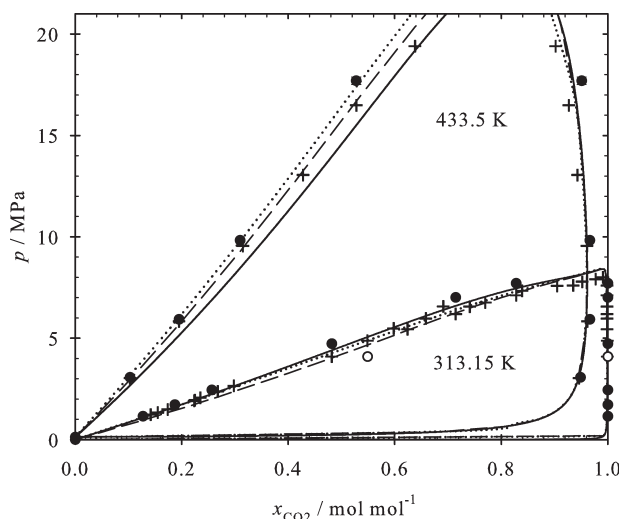
Figure 7. Isothermal vapor-liquid phase diagram of carbon dioxide + cyclohexanone at 313.15 and 433.5 K: + experimental data 5,8,69,70 ; ○ present simulation data with \xi = 1 ; ● simulation data with \xi = 0.985 ; - - COSMO-SAC; — COSMO-SAC with I_{ij} = -0.0082 ; ... PR EOS with k_{ij} = 0.049 .
