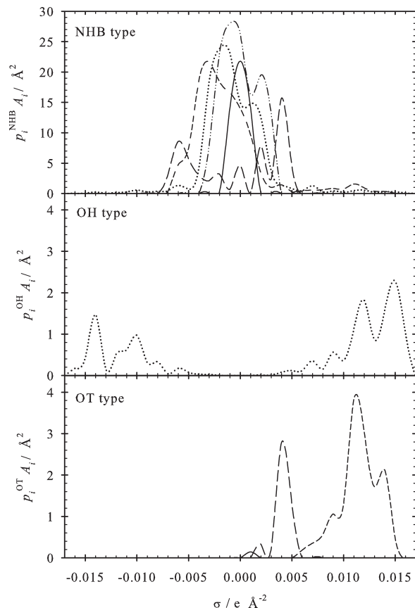
Figure 1. The \sigma -profiles of the five regarded components of NHB type (top), OH type (center), and OT type (bottom): — oxygen; — — carbon dioxide; - ... cyclohexane; - - cyclohexanone; ... cyclohexanol.
