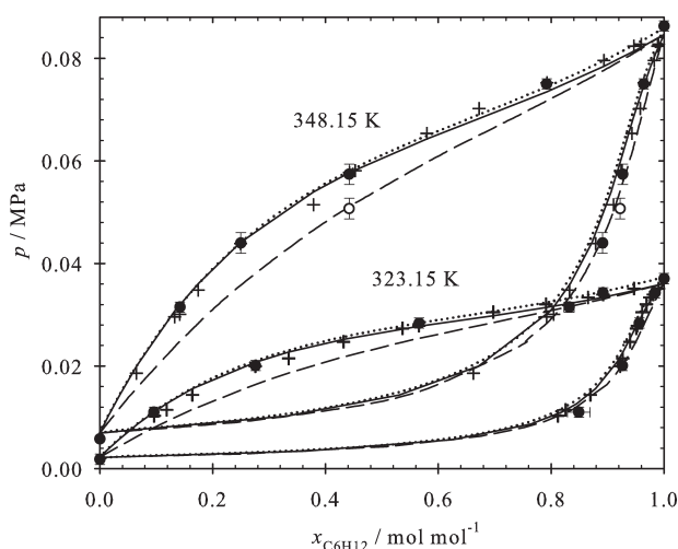
Figure 9. Isothermal vapor-liquid phase diagram of cyclohexane + cyclohexanone at 323.15 and 348.15 K: + experimental data 47 ; o present simulation data with \xi = 1 ; • simulation data with \xi = 0.98 6 ; - - COSMO-SAC; — COSMO-SAC with l_{ij} = -0.0228 ; ... PR EOS with k_{ij} = 0.065 .
